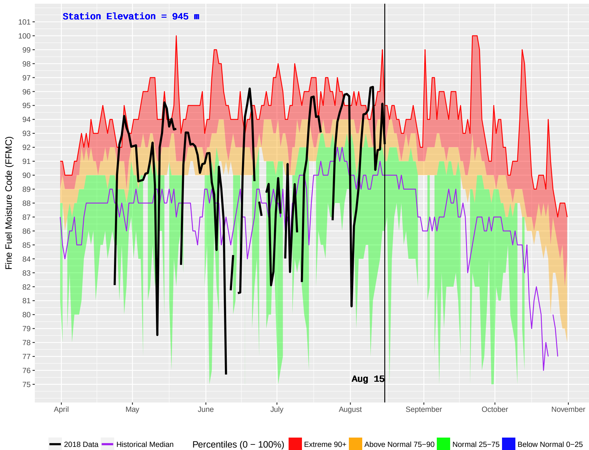
TATLA LAKE HUB (208) : Historical (1980–2016) and Current (2018) Daily Fine Fuel Moisture Code (FFMC)
